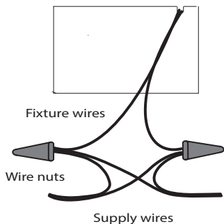
WIRING DIAGRAM
